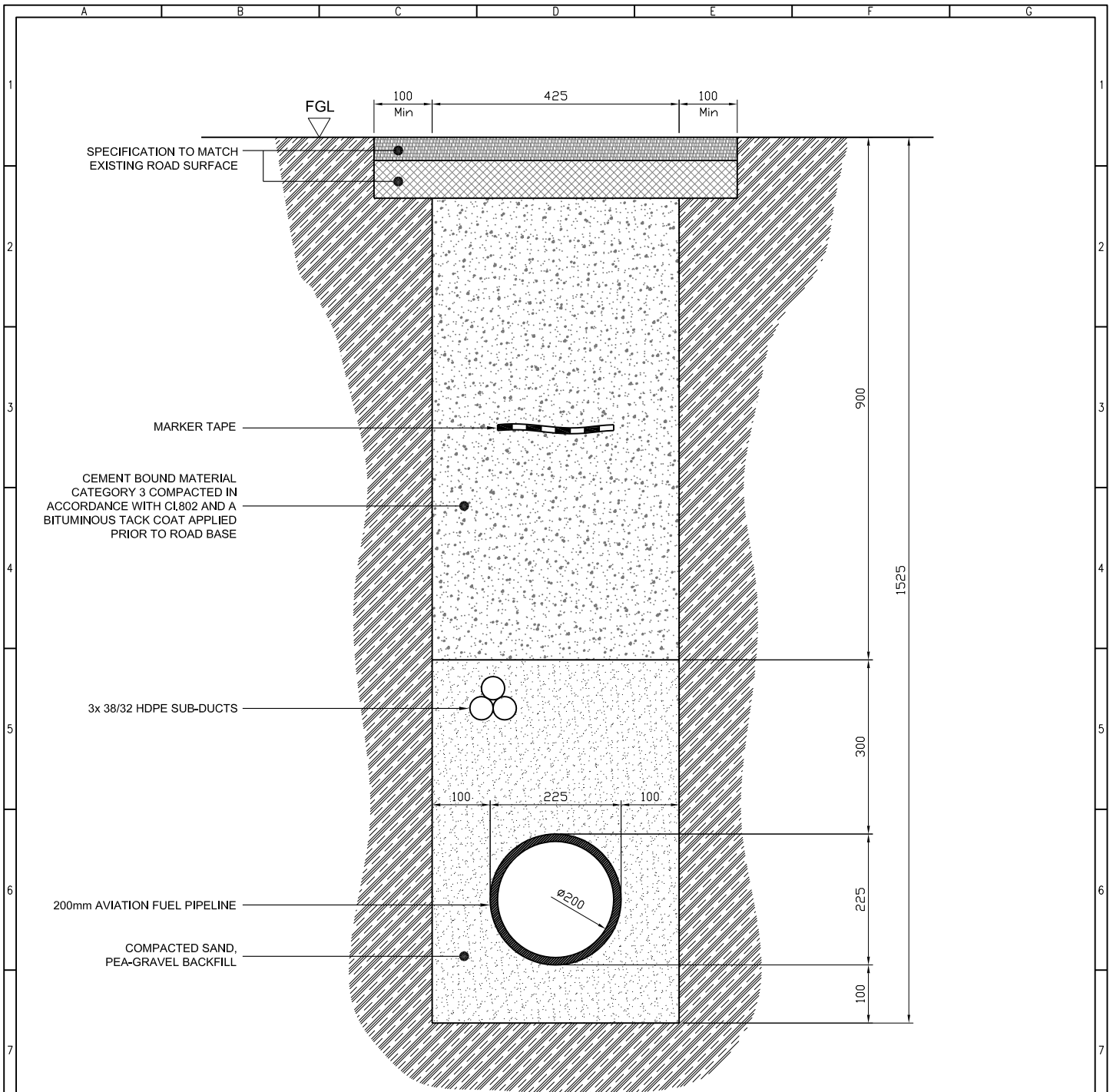
TYPICAL CROSS SECTION OF PIPELINE TRENCH
